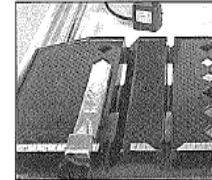
(E) Position the Adjustable Cutting Guide to desired cut length
