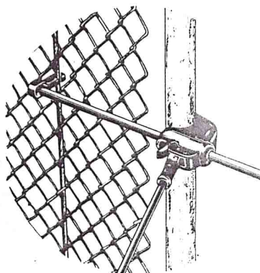
Model A Used with Tension Bar For Stretching Fabric
