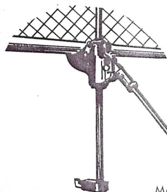
Model A with Workhead Reversed For Lifting Gates or Panels
